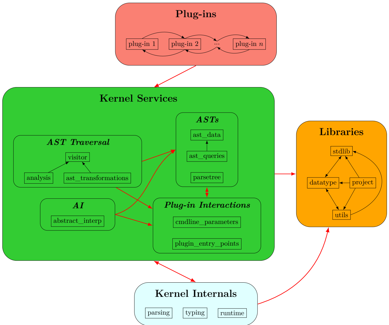
Figure 3.1: Frama-C Architecture Design.
